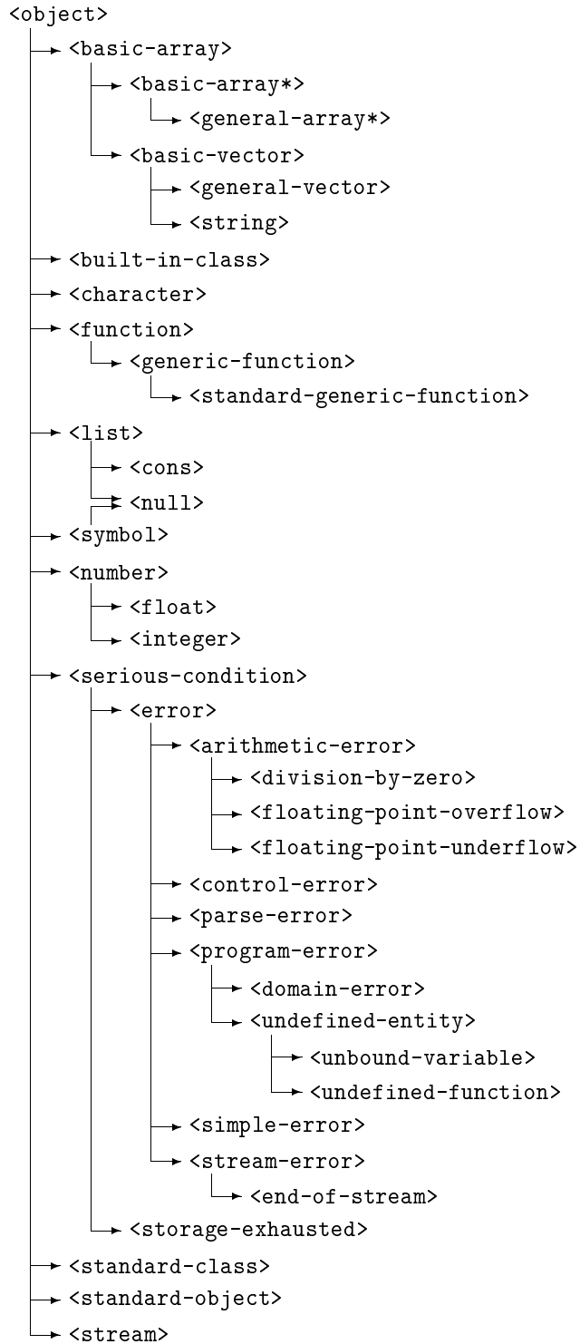
Figure 1. Class Inheritance
